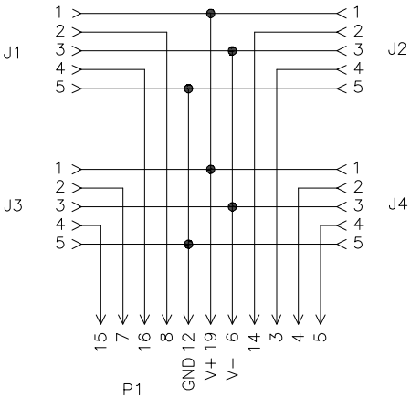
WIRING DIAGRAM
